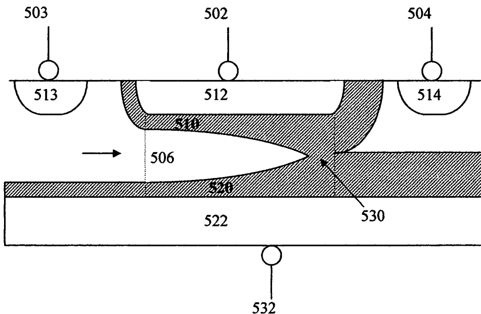
FIG-5 (Prior Art)
